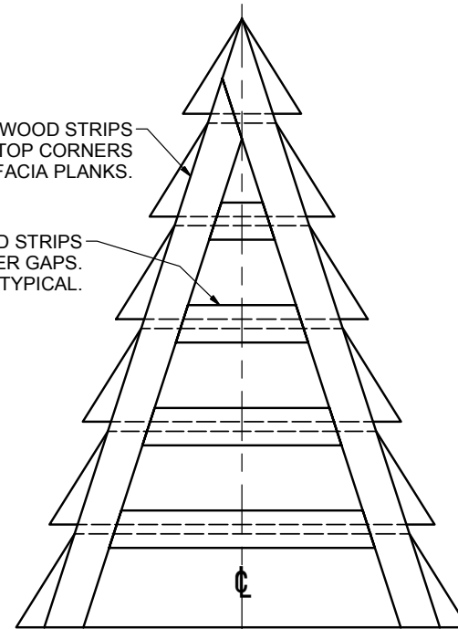
② SMALLER TREE - BACK 1"=1'-0" 3 REQUIRED
