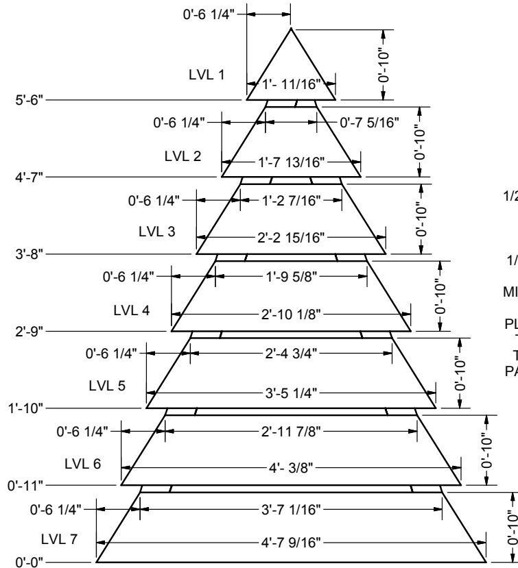
1 PLANK TREE - FACE 1"=1'-0" 2 REQUIRED
