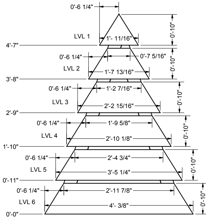
① SMALLER TREE - FACE 1"=1'-0" 3 REQUIRED
