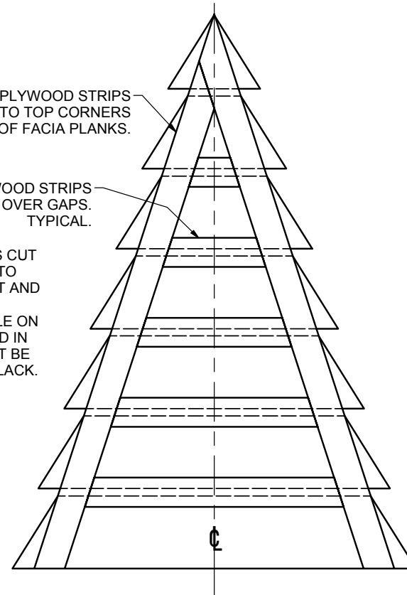
2 PLANK TREE - BACK 1"=1'-0" 2 REQUIRED
